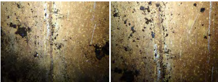
Middle North Wall Section- Photo of weld deficiencies
