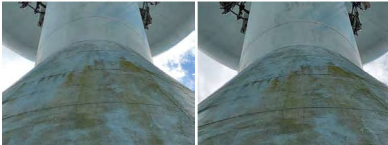
Upper North Wall Section- Photo of weld deficiencies
