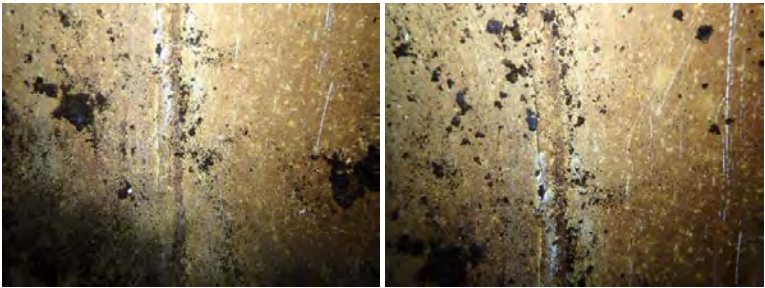
Middle North Wall Section- Photo of weld deficiencies
